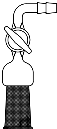
Adapter , Flow Control , Glass Stopcock , 90° With standard taper outer joint and hose connection
